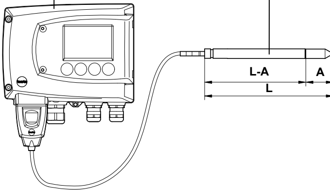
testo 6604/6605 cable probe
