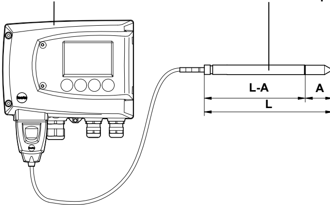
testo 6681 transmitter
